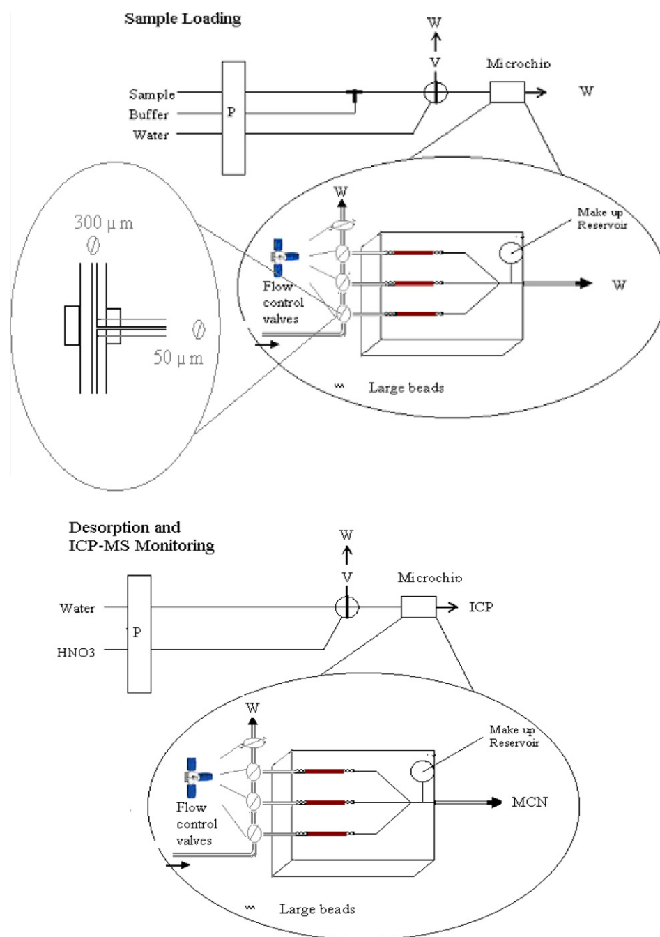
Figure 4 Flow injection manifolds for trace metals sample loading, and desorption and monitoring. P, peristaltic pump; V, flow selection valve; W, waste; MCN, micro-concentric nebuliser; V, flow selection valve; ICP, inductively coupled plasma.
