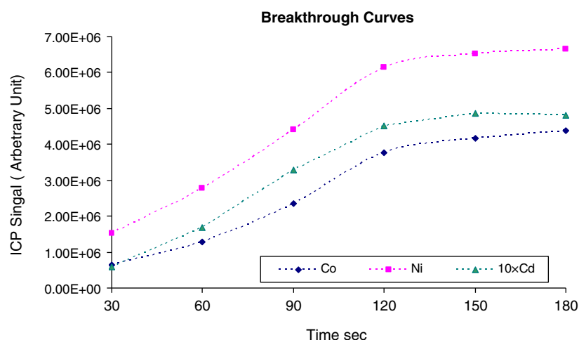
Figure 7 Breakthrough of the packed microchannel obtained using standard solutions of 20 \text{ ng ml}^{-1} of Cd, Co, and Ni loaded at 20 \mu\text{l min}^{-1} .
