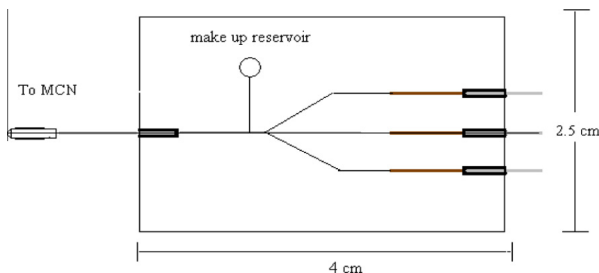
Figure 1 Schematic diagram for the microfluidic device with three packed microchannels (brown lines) and the glued connection PTFE tubing for its coupling with FI and the interface with ICP-MS.
