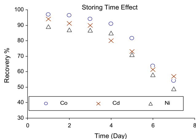
Figure 8 Effect of storing time on metals recovery.
