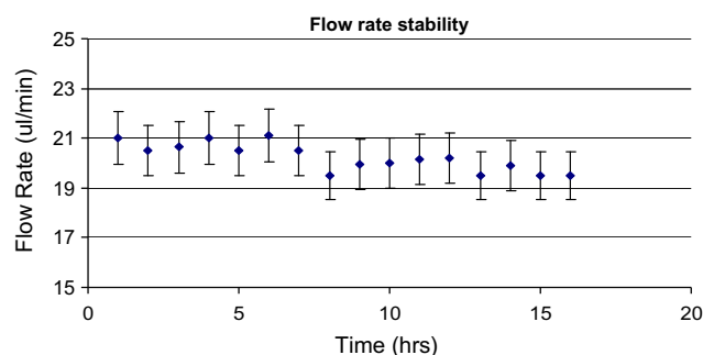
Figure 5 Flow rate stability at 20 \mu\text{l min}^{-1} maintained by splitting the main stream using a controlling valve.
