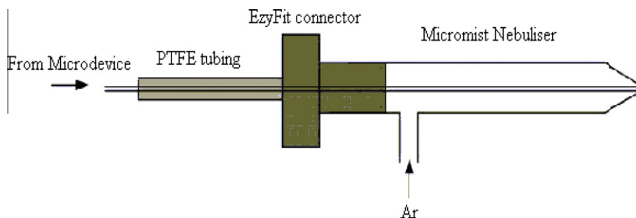
Figure 3 Schematic diagram of microchip-ICP interface (Song et al., 2003).
