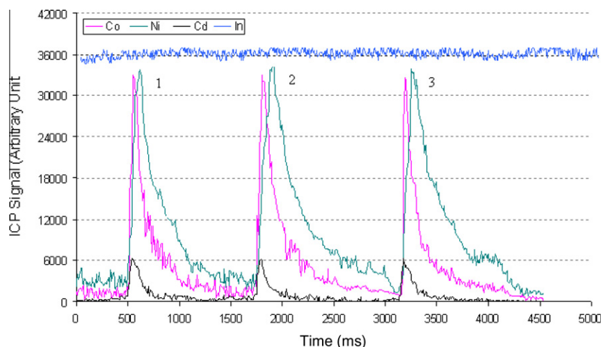
Figure 6 Multielement scans showing the elution profiles for studied metals in standard solutions containing 5 \text{ ng ml}^{-1} loaded for 90 s. Also shown is the stable baseline signal from 50 \text{ ng ml}^{-1} internal standard, In.
