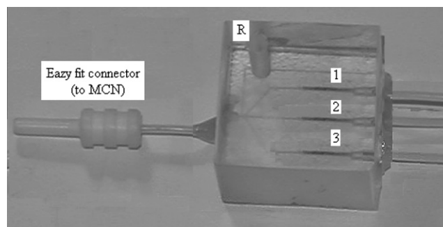
Figure 2 Photograph of the microfluidic device; 1, 2, and 3 indicate the packed microchannels; R, make up reservoir. The photo shows the glued connection PTFE tubing to interface the devices with the ICP and the FI manifold.
